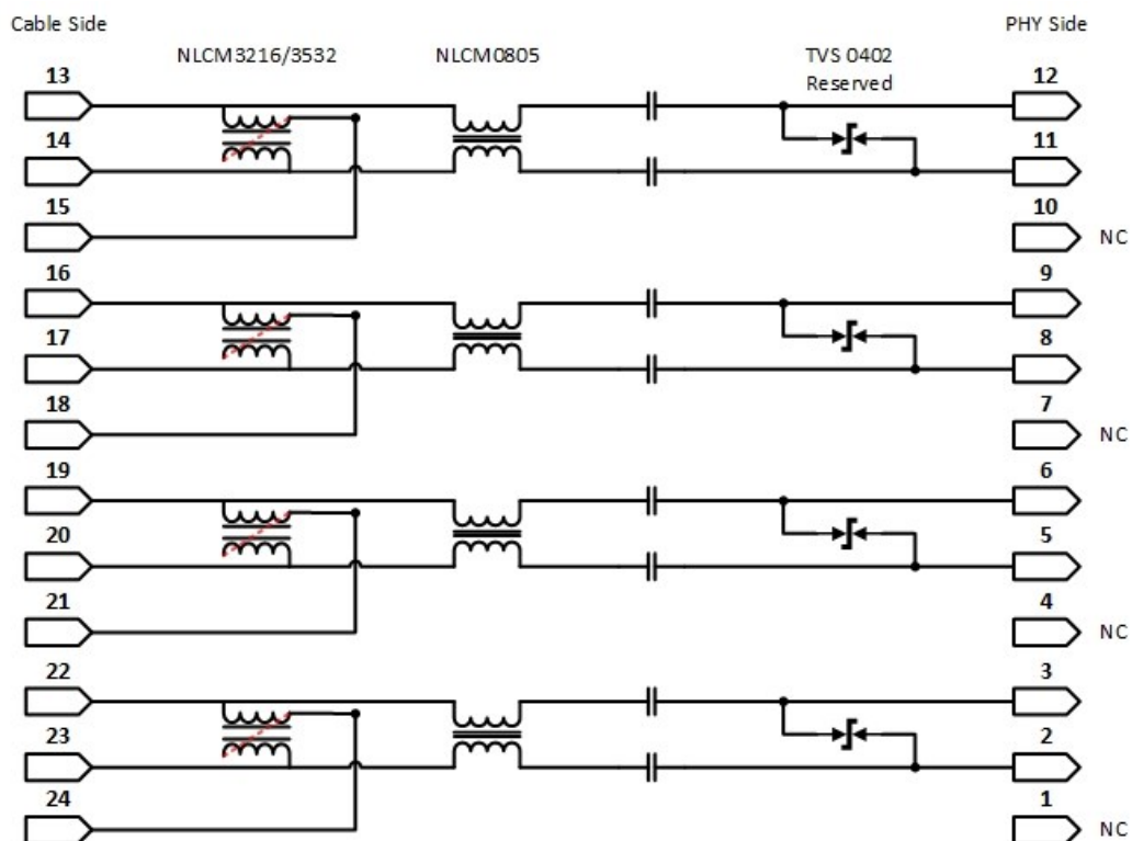
Fig.3 Typical Application
