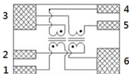
Fig.1 Pin Configuration
