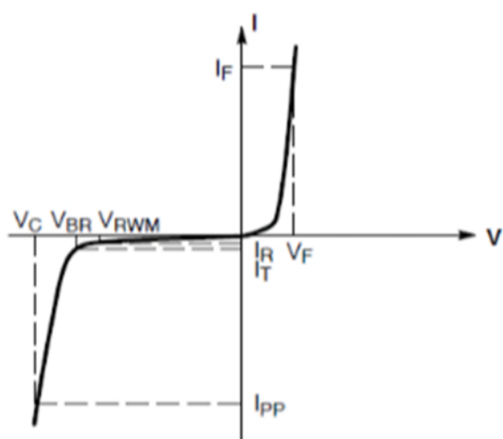
Figure1. I-V Characteristics
