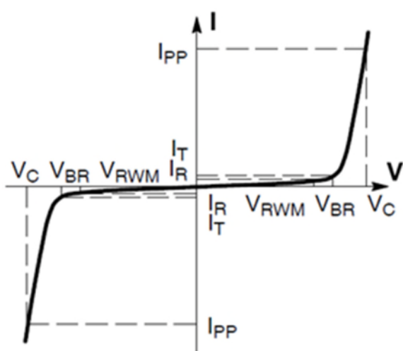
Figure1. I-V Characteristics
