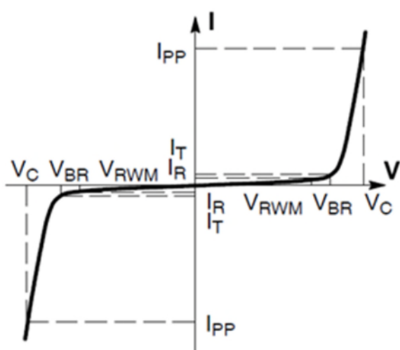
Figure1. I-V Characteristics
