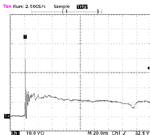
Figure1. Clamping waveform of positive 8KV ESD contact
